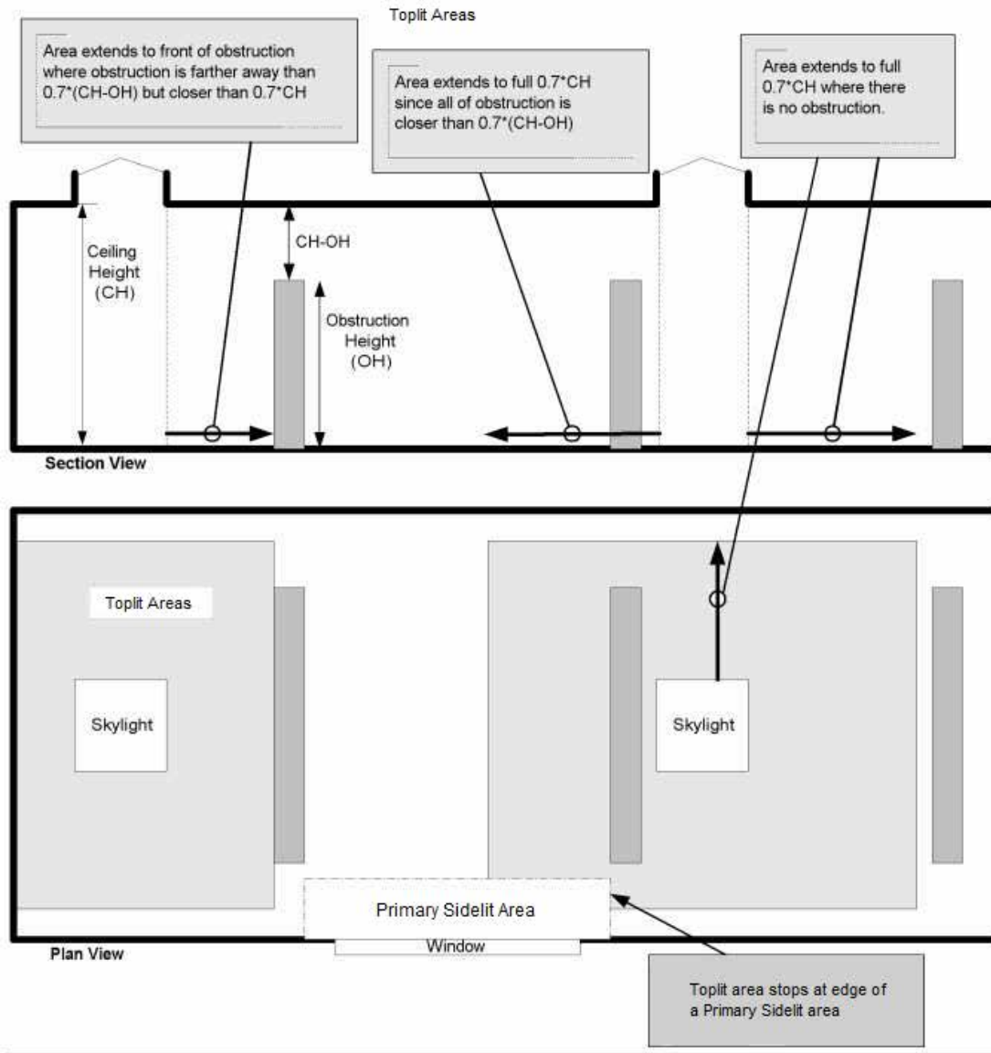
FIGURE C405.2.4.3(1) TOPLIT ZONE UNDER A ROOFTOP FENESTRATION ASSEMBLY
